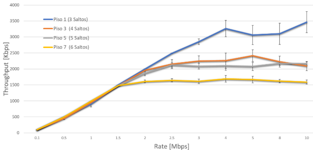
Figura 6 Throughput [Kbps] vs data rate deseado [Mbps]
