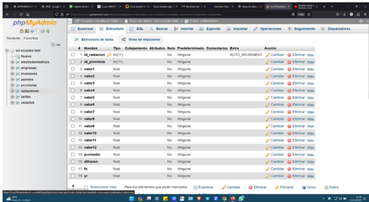
Fig. 4. Database configuration
