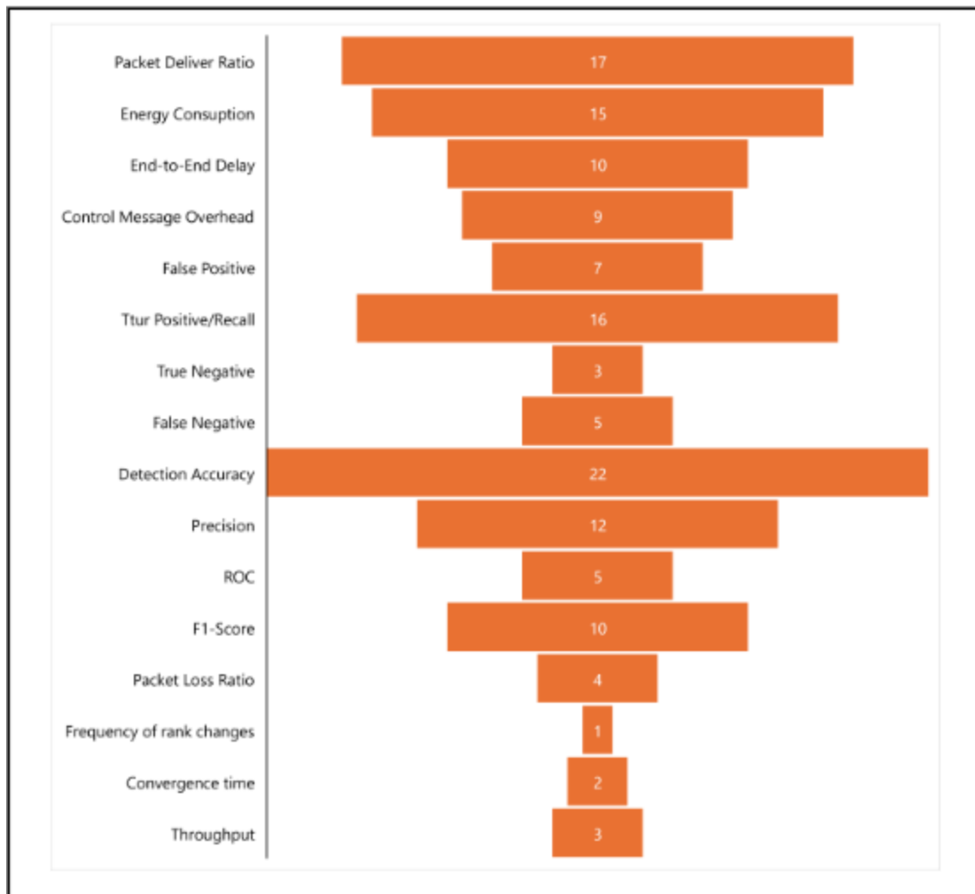
Fig. 8 Occurrence of evaluation metrics in selected studies
