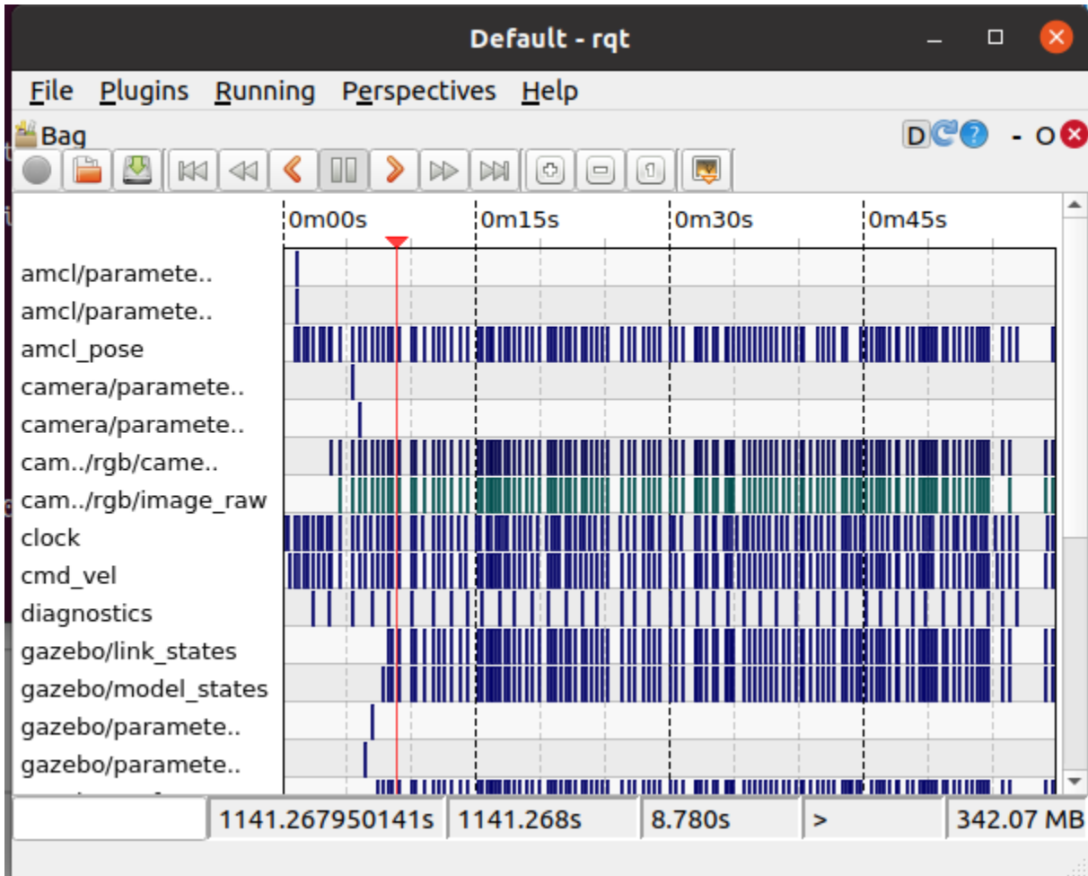
Fig. 4. An example of rqt bag.
