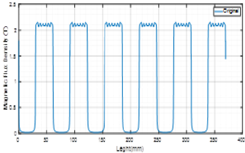
FIG. 8. Magnetic flux density for peak current of original motor
