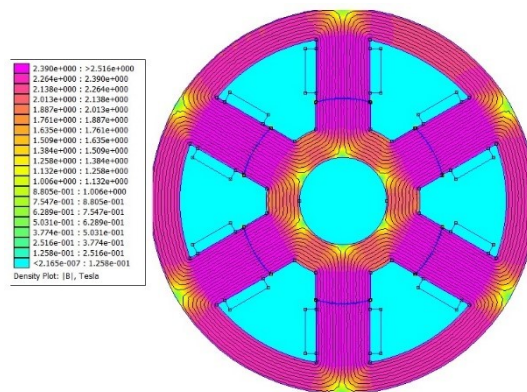
FIG. 3 Original motor aligned
