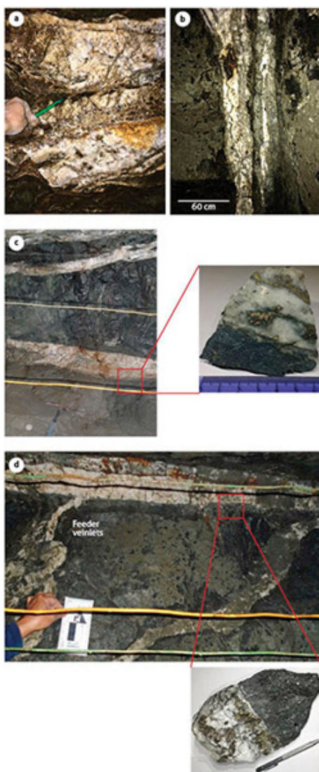
FIGURE 8. E-W striking extension veins observed in the El Apique mine a-b-c) Quartz-calcite extension vein. d) Mineralized igneous body with chloritization cut by quartz-calcite veins with chalcopyrite, pyrite and sphalerite.
