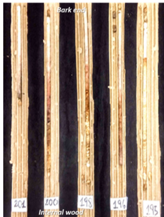
FIGURE 4 Wood samples with rot with pinkish and greyish coloration
