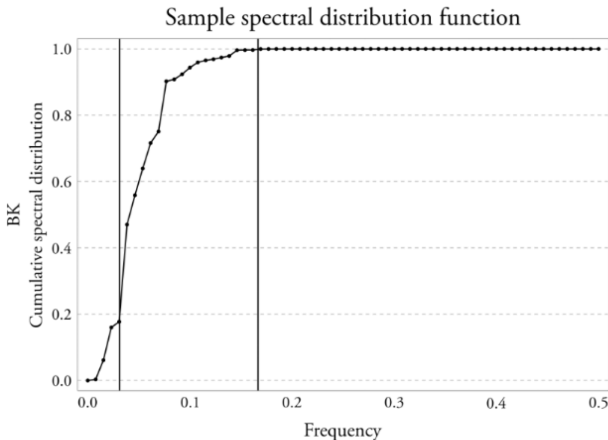
FIGURE 23 Cumulative spectral distribution — BK
