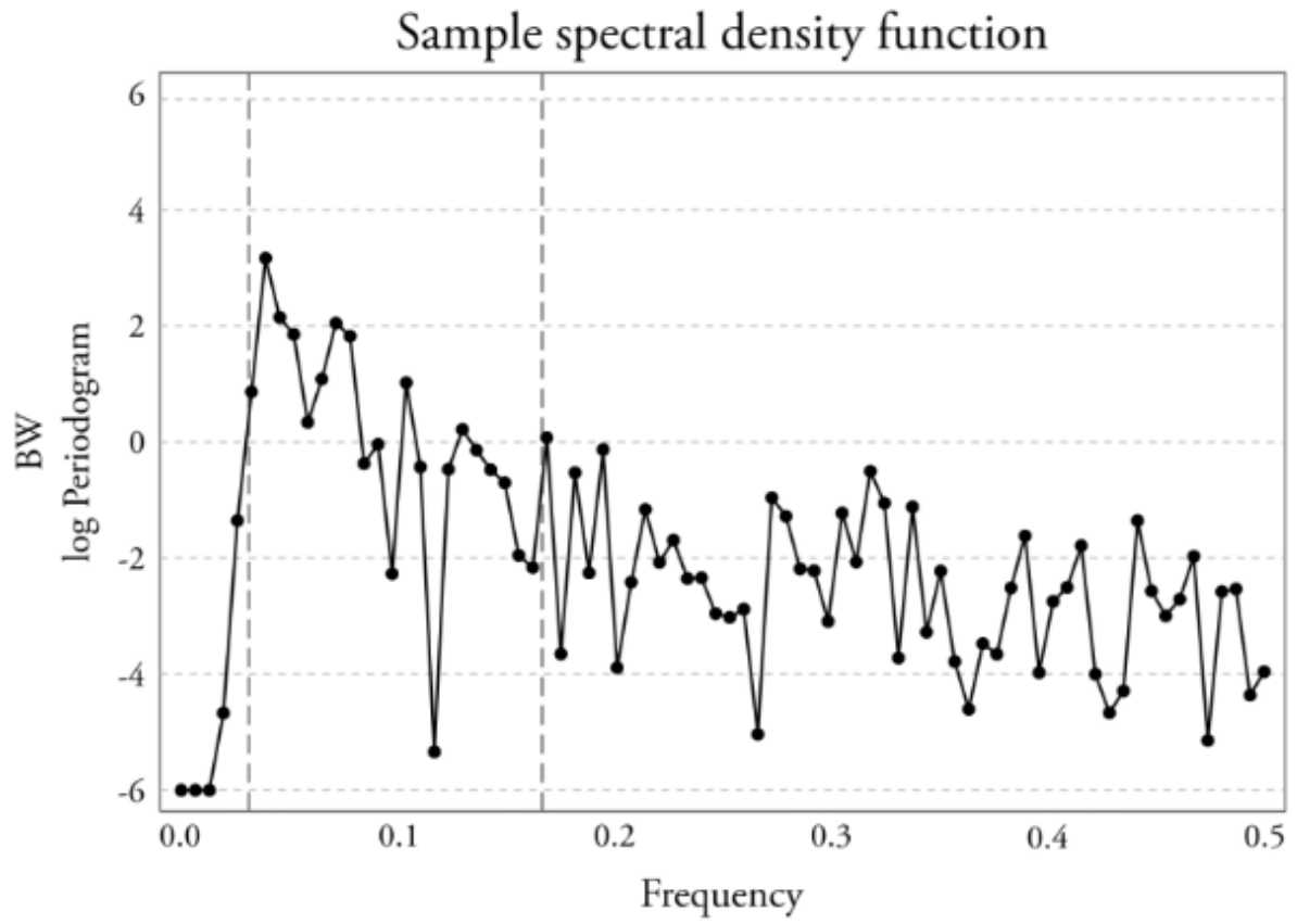
FIGURE 17 Sample spectral density of BW cycle
