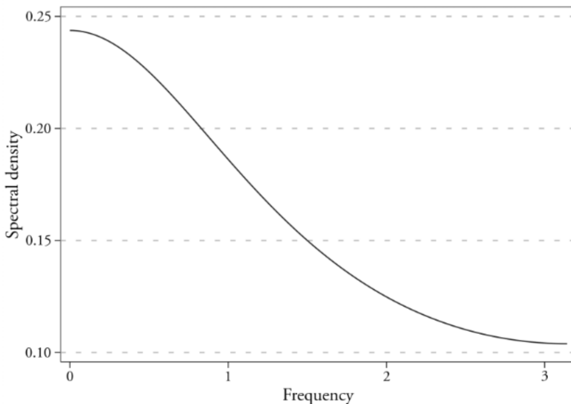
FIGURE 6 Spectral density of Argentina's quarterly GDP
