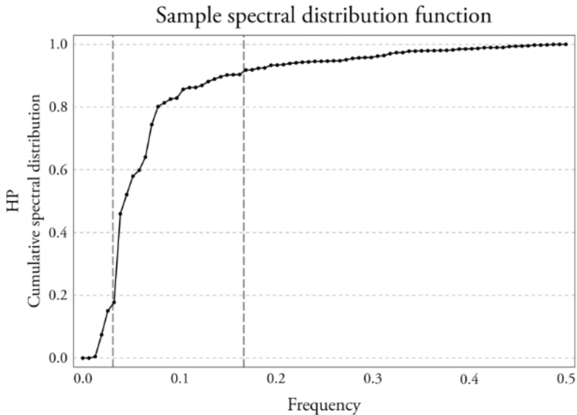
FIGURE 20 Cumulative spectral distribution – HP
