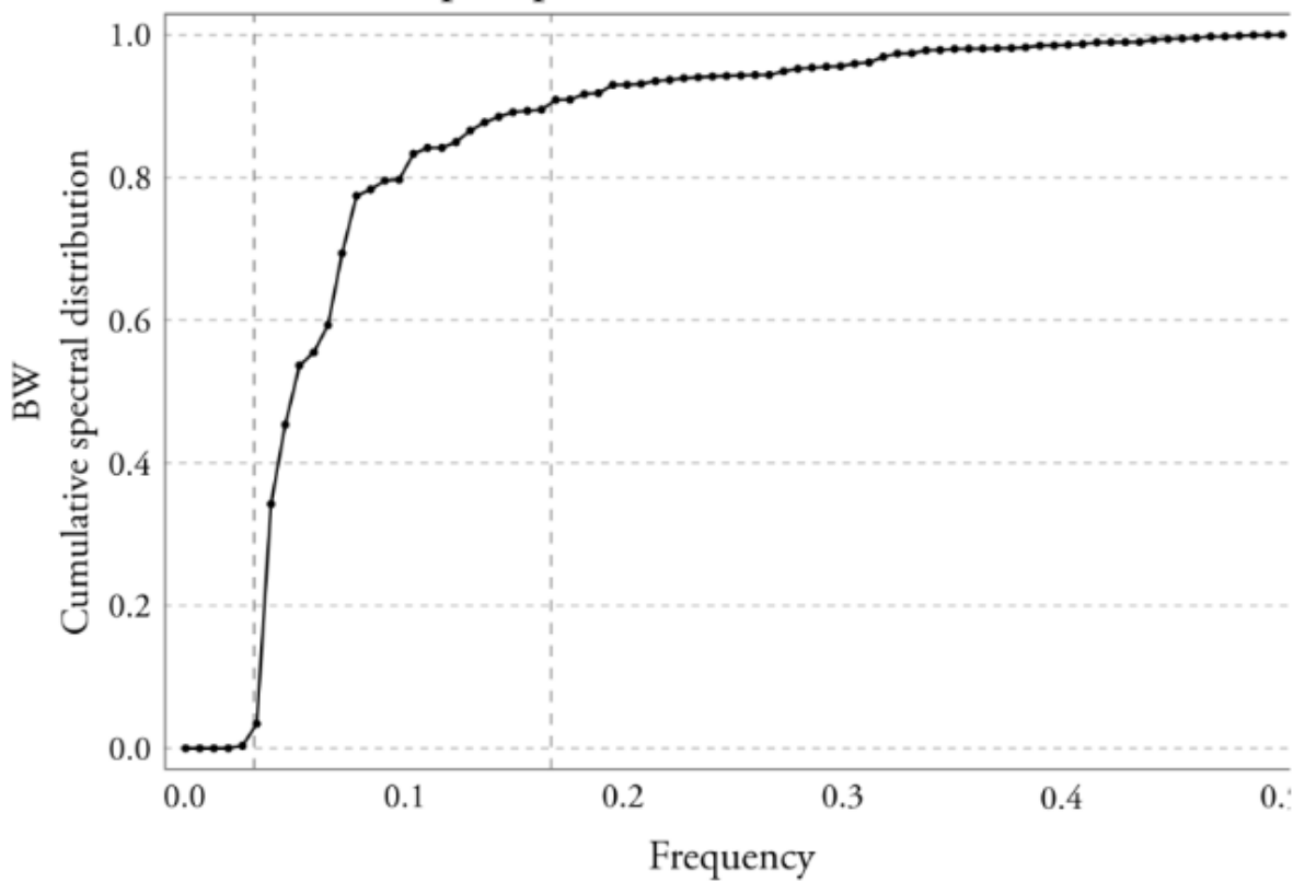
FIGURE 22 Cumulative spectral distribution — BW Sample spectral distribution function
