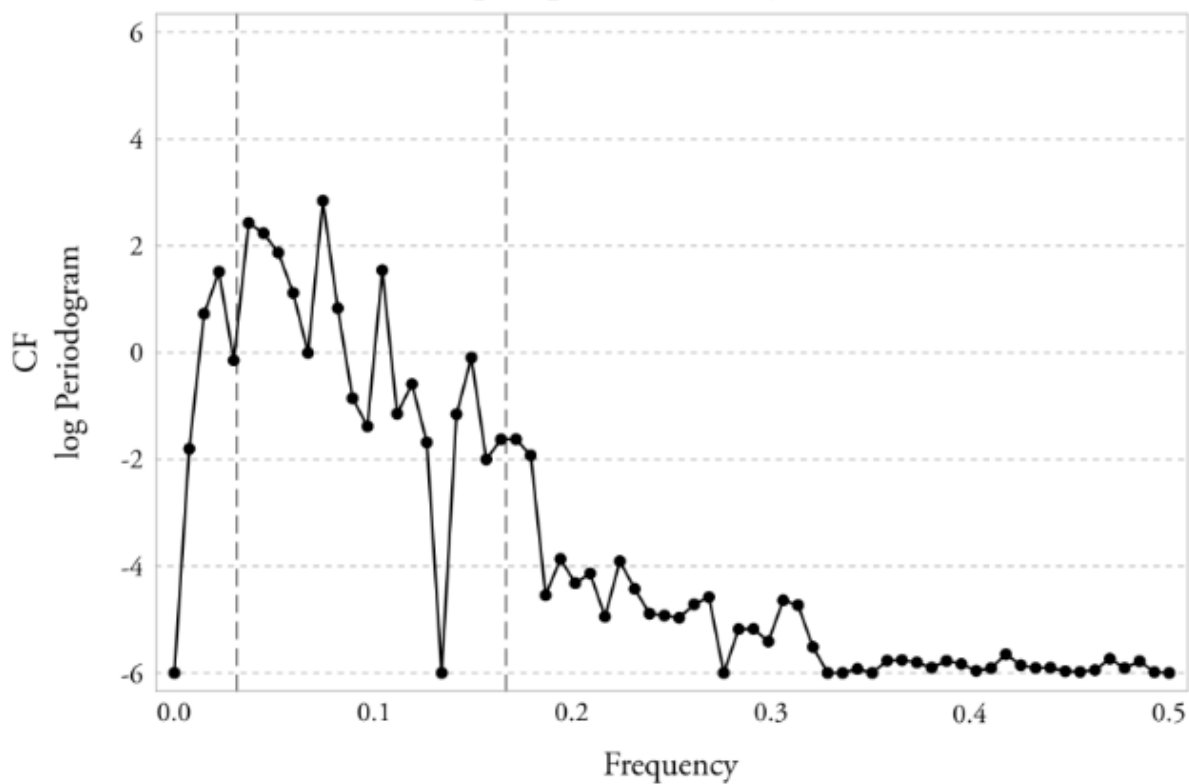
FIGURE 16 Sample spectral density of CF cycle Sample spectral density function
