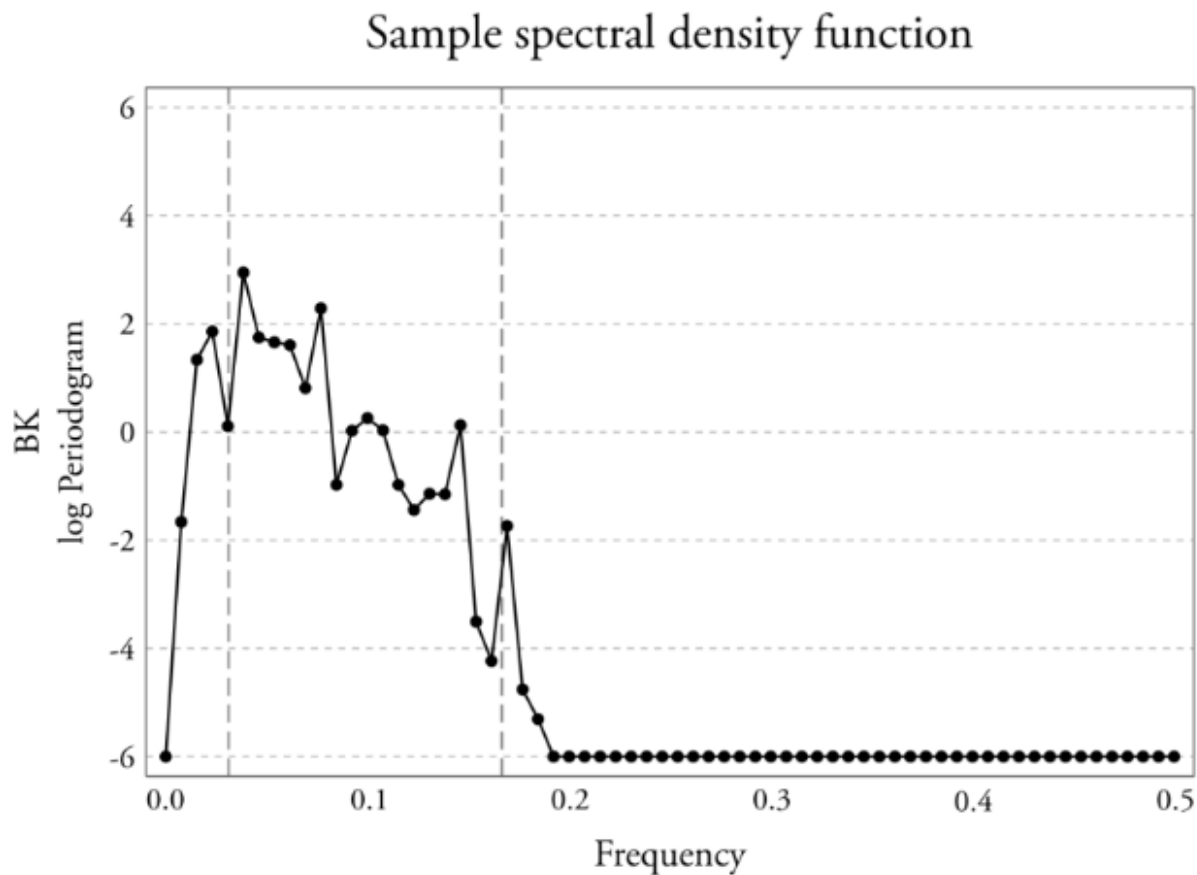
FIGURE 18 Sample spectral density of BK cycle.
