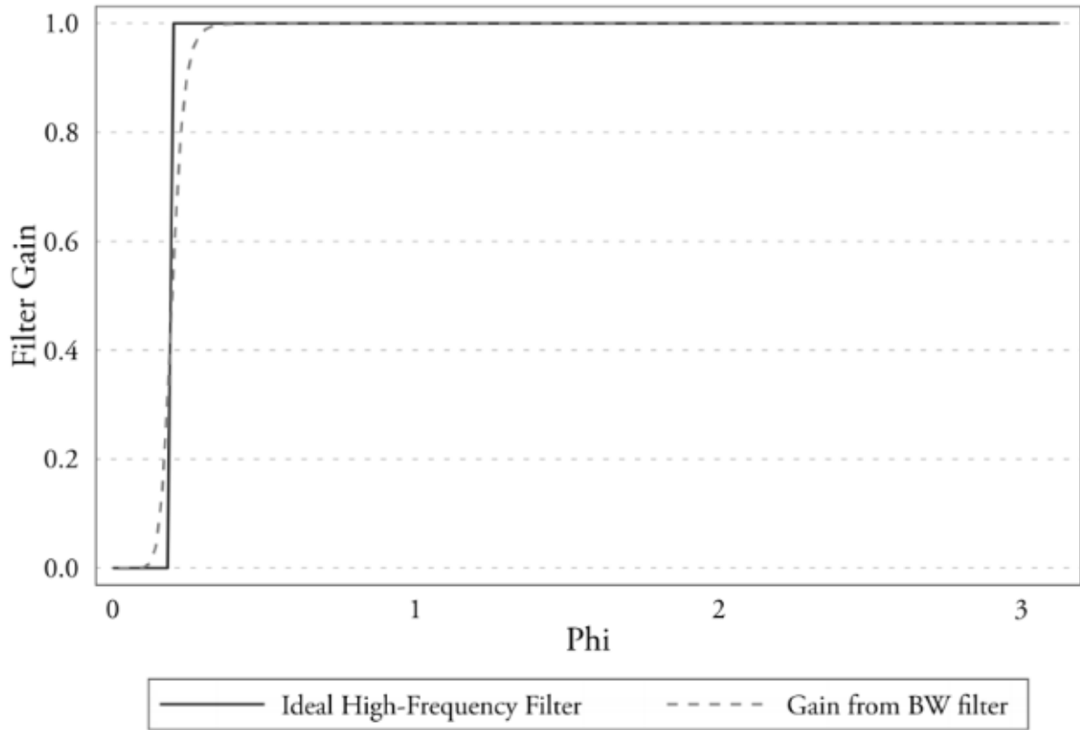
FIGURE 13 Gain of the Butterworth filter
