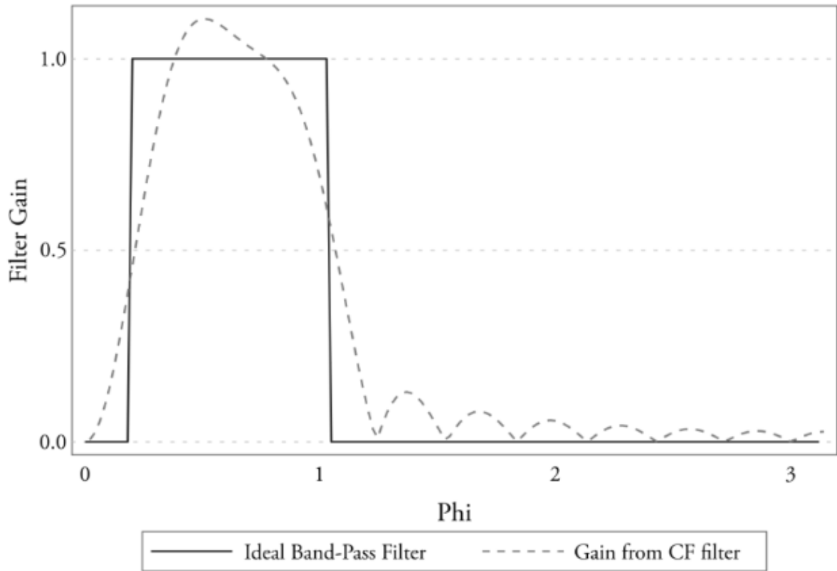
FIGURE 12 Gain of the Christiano-Fitzgerald filter
