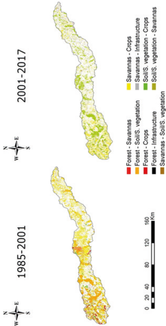
Figure 6. Land-cover change of the Bitá river basin in the periods: 1985-2001 and 2001-2017
